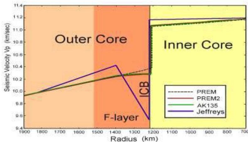
Figure 4. Variation chart of seismic wave velocity in the F-layer: V_p low-velocity gradient and sharp-velocity discontinuity at the ICB indicate their different components.
