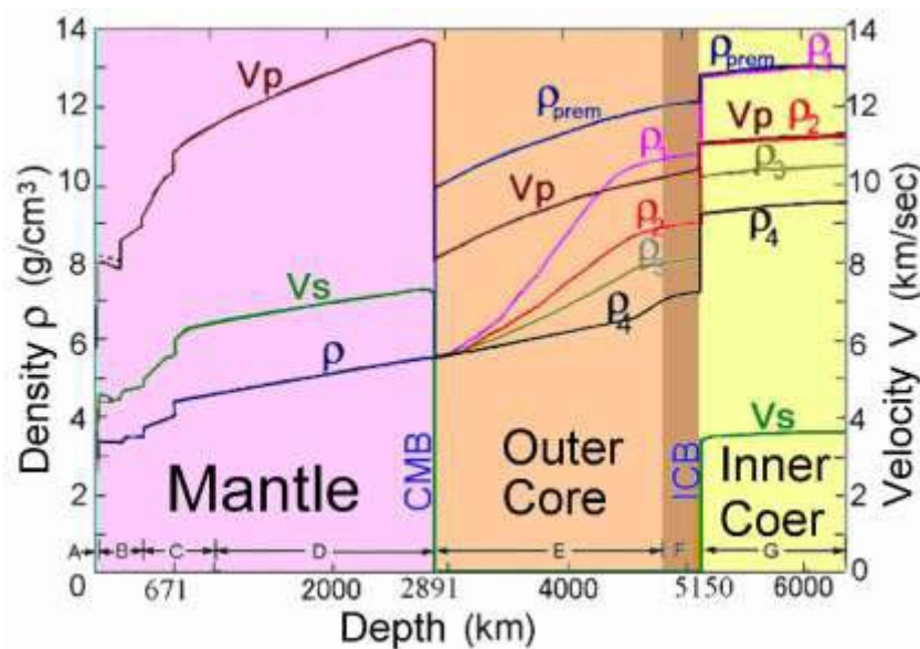
Figure 7. These densities \rho of the new Earth models 1, 2, 3, and 4 were compared with those of the PREMs.
