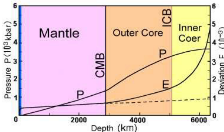
Figure 6. The pressure P of the PREM and the deviation E of the calculated pressure using the simplified method
