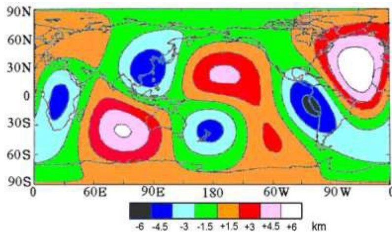
Figure 3. The topography of the CMB obtained by inversion of the combined PcP and PKPBC dataset.
