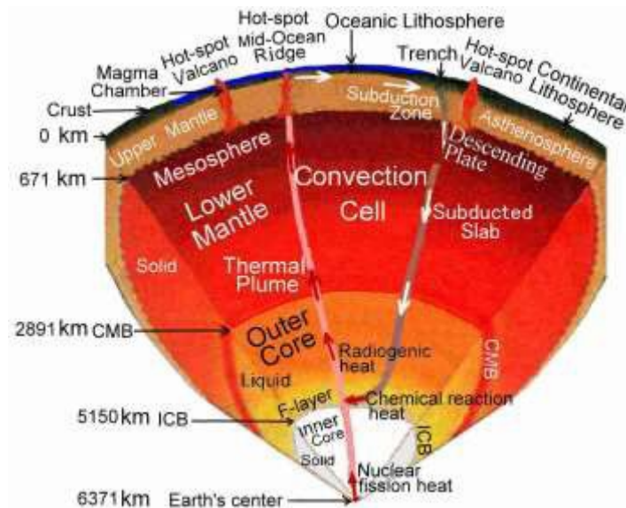
Figure 5. Schematic diagram of the great convection cell, heat flow and composition of the Earth's interior.
