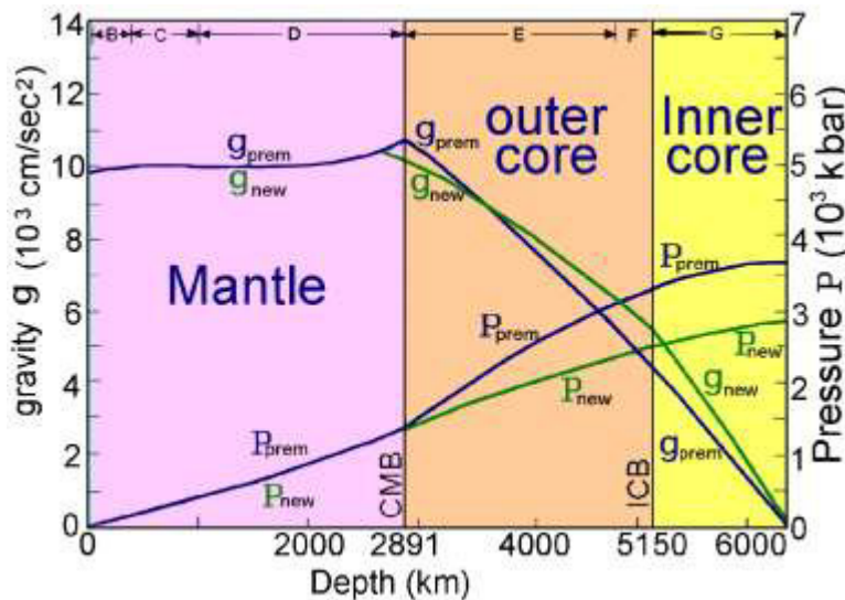
Figure 8. Diagram of the gravity g and the pressure P of the new Earth model compares to PREM.
