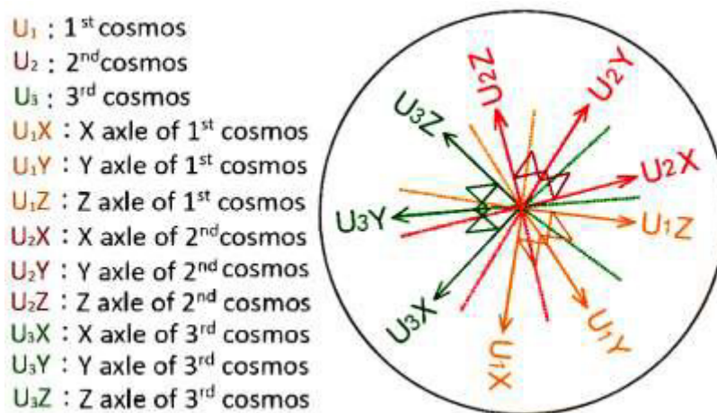
Figure1. Schematic representation of nine-dimensional space in 3-cosmic framework of the universe.
