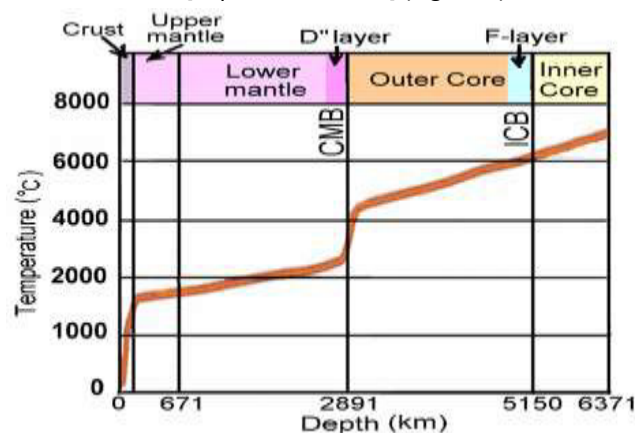
Figure 2. The temperature profile of the Earth's interior
